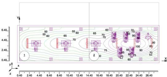
Lighting System
